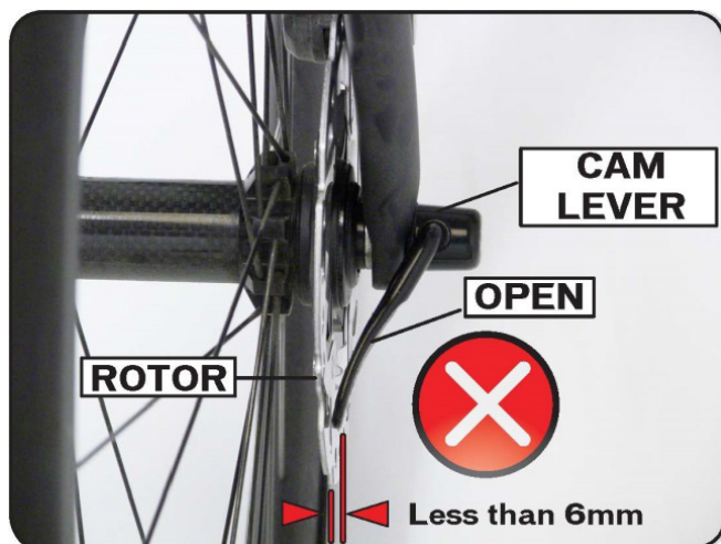
Fig. 1: Quick-release lever with potential for contact
