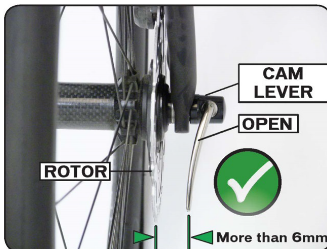
Fig. 2: Quick-release lever with adequate clearance
